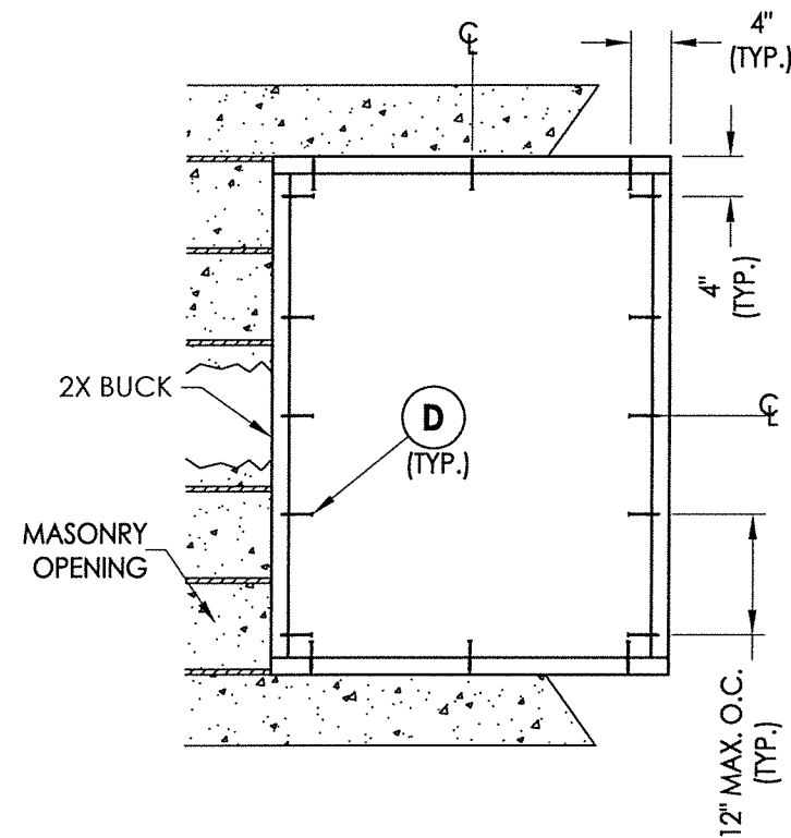
BUCK ANCHORING 36" x 48" MAX. FRAME SIZE DESIGN PRESSURE > +70.0 / -70.0 PSF
