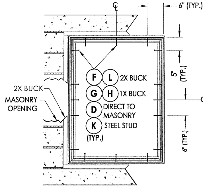
FRAME ANCHORING 36" x 48" MAX. FRAME SIZE DESIGN PRESSURE > +70.0 / -70.0 PSF
